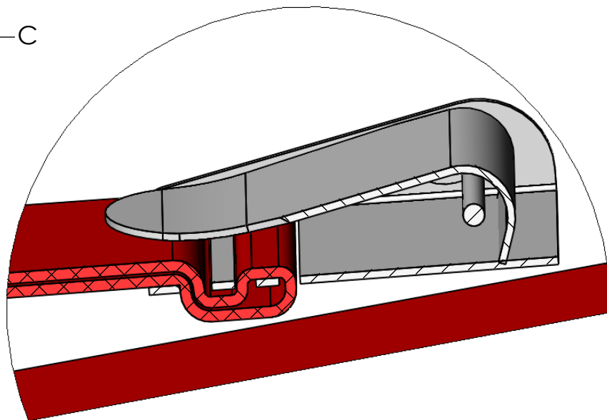
Detail C
